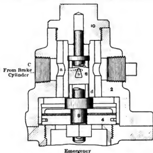
Fig. 2504. High-Speed Reducing Valve. Emergency Position.
